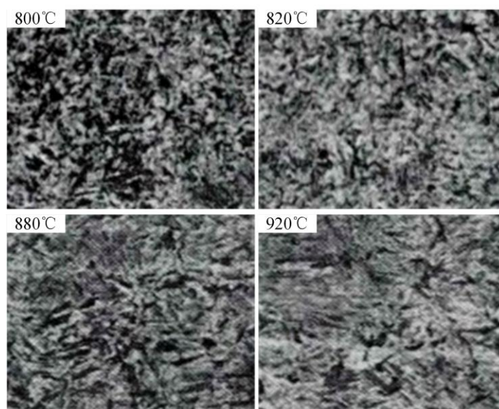
Figure 1. Microstructure of 50CrMnVA experimental steel after quenching at different temperatures and tempering at 490 °C
