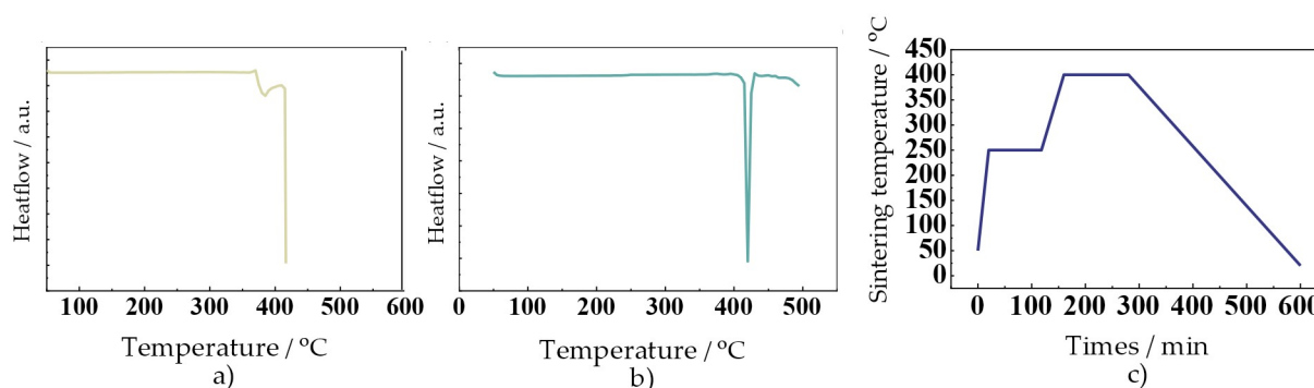
Figure 1. Differential scanning calorimetry (DSC) and sintering process curves of powder mixtures of a) Zn, b) Mg, and c) Mn
