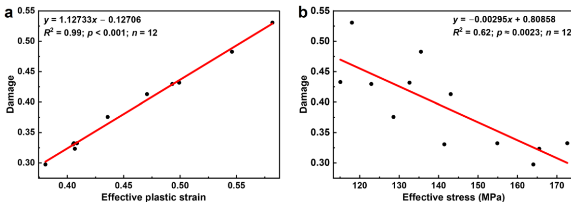
Figure 13. Relationships between final Damage and (a) final effective plastic strain and (b) final effective stress at point P, across 12 unique simulation conditions. Linear regression results (equation, R^2 , and p -value) are given within each panel
