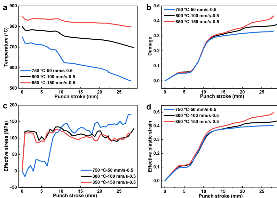
Figure 10. Evolution of temperature, Damage, effective stress, and effective plastic strain at point P with punch stroke under different die-entry temperature–punch speed combinations (750 °C–50 mm·s -1 , 800 °C–100 mm·s -1 , and 850 °C–150 mm·s -1 ) at a friction coefficient of 0.5: (a) temperature; (b) Damage; (c) effective stress; (d) effective plastic strain
