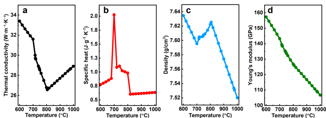
Figure 2. Temperature-dependent thermophysical parameters of 22MnB5 high-strength steel calculated using JMatPro software: thermal conductivity (a); specific heat (b); density (c); Young's modulus (d)
