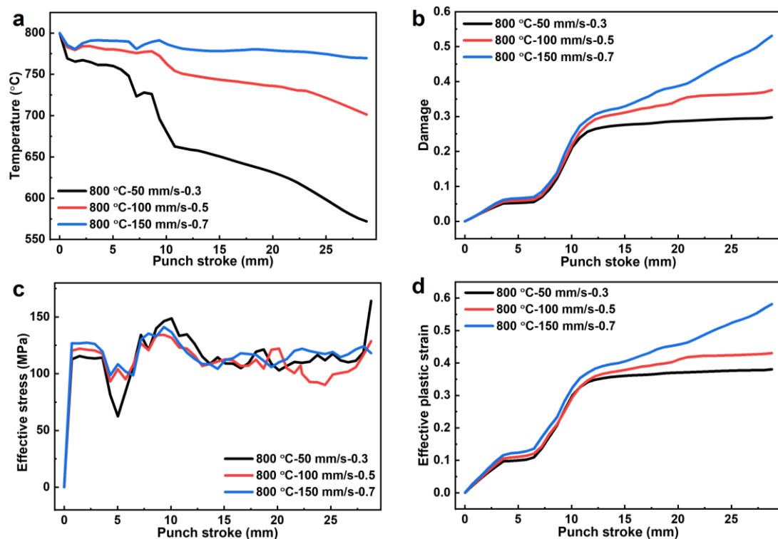
Figure 12. Evolution of temperature, Damage, effective stress, and effective plastic strain at point P with punch stroke under different punch speed–friction coefficient combinations (50 mm·s -1 –0.3, 100 mm·s -1 –0.5, and 150 mm·s -1 –0.7) at a die-entry temperature of 800 °C: (a) temperature; (b) Damage; (c) effective stress; (d) effective plastic strain
