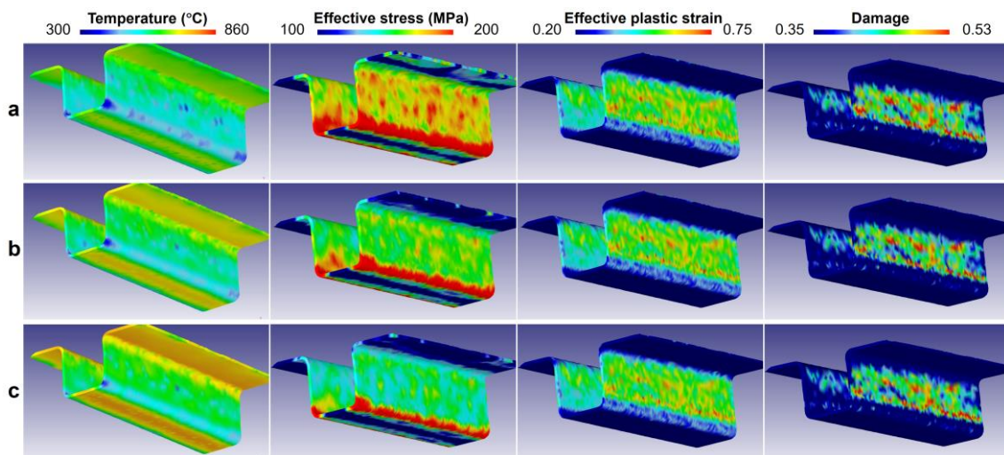
Figure 4. Effect of die-entry temperature on the thermo-mechanical response and damage distribution of the 22MnB5 hot-stamped component at a punch speed of 50 mm·s -1 and a friction coefficient of 0.5: (a) 750 °C; (b) 800 °C; (c) 850 °C
