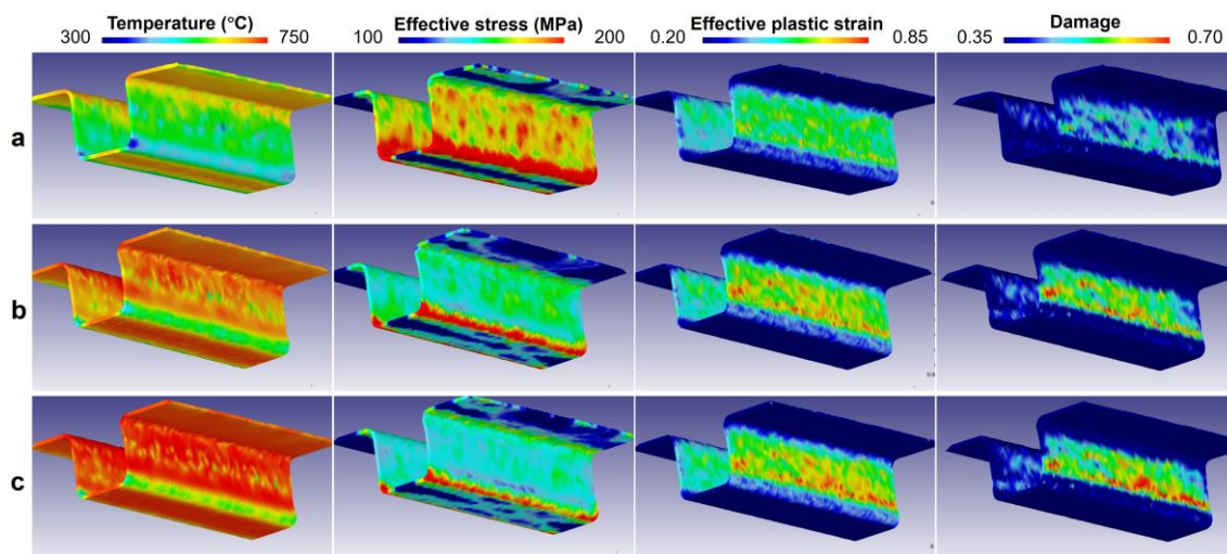
Figure 6. Effect of punch speed on the thermo-mechanical response and damage distribution at a die-entry temperature of 750 °C and a friction coefficient of 0.5: (a) 50 mm·s -1 ; (b) 100 mm·s -1 ; (c) 150 mm·s -1
