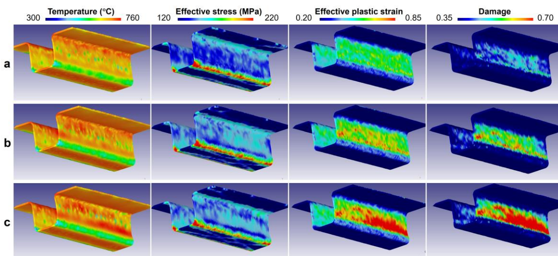
Figure 8. Effect of friction coefficient on the thermo-mechanical response and damage distribution of the 22MnB5 hot-stamped component at a die-entry temperature of 750^\circ\text{C} and a punch speed of 100 \text{ mm}\cdot\text{s}^{-1} : (a) 0.3; (b) 0.5; (c) 0.7
