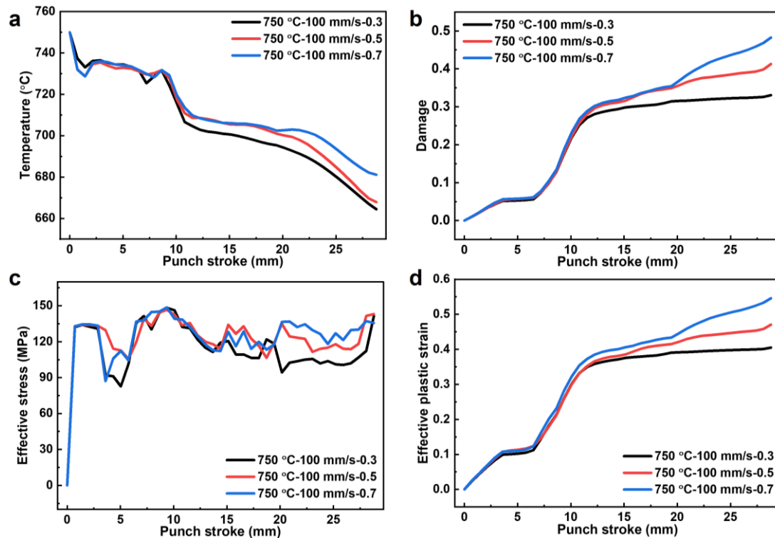
Figure 9. Evolution of temperature, Damage, effective stress, and effective plastic strain at point P with punch stroke under different friction coefficients (0.3, 0.5, and 0.7) at a die-entry temperature of 750 °C and a punch speed of 100 mm·s -1 : (a) temperature; (b) Damage; (c) effective stress; (d) effective plastic strain
