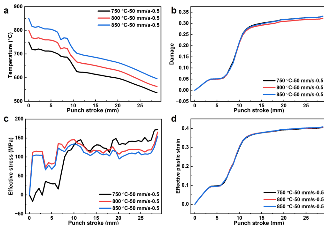
Figure 5. Evolution of temperature, Damage, effective stress, and effective plastic strain at point P with punch stroke under different die-entry temperatures (750 °C, 800 °C, and 850 °C) at a punch speed of 50 mm·s -1 and a friction coefficient of 0.5: (a) temperature; (b) Damage; (c) effective stress; (d) effective plastic strain
