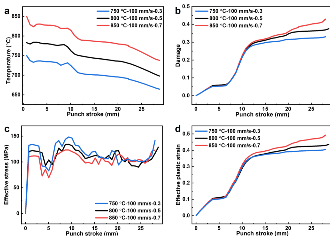
Figure 11. Evolution of temperature, Damage, effective stress, and effective plastic strain at point P with punch stroke under different die-entry temperature–friction coefficient combinations ( 750^\circ\text{C}-0.3 , 800^\circ\text{C}-0.5 , and 850^\circ\text{C}-0.7 ) at a punch speed of 100 \text{ mm}\cdot\text{s}^{-1} : (a) temperature; (b) Damage; (c) effective stress; (d) effective plastic strain
