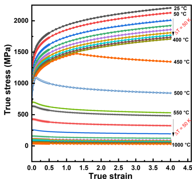
Figure 3. True stress–strain curves of 22MnB5 high-strength steel at different temperatures calculated using JMatPro
