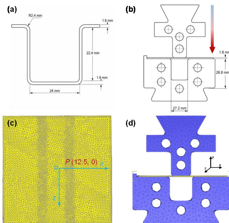
Figure 1. Dimensions of the simulated hot-stamping component (a); relative positions of the punch, die, and blank with corresponding forming dimensions (b); mesh discretization of the blank (c); and overall mesh discretization of the punch–die–blank assembly (d)
